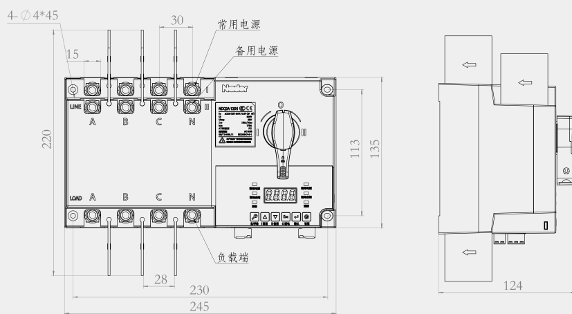
NDQ2A-125H
